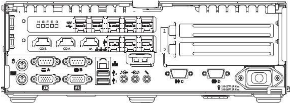
Figure 2: IBM 4800 Back (with Second SurePORT Shown)
