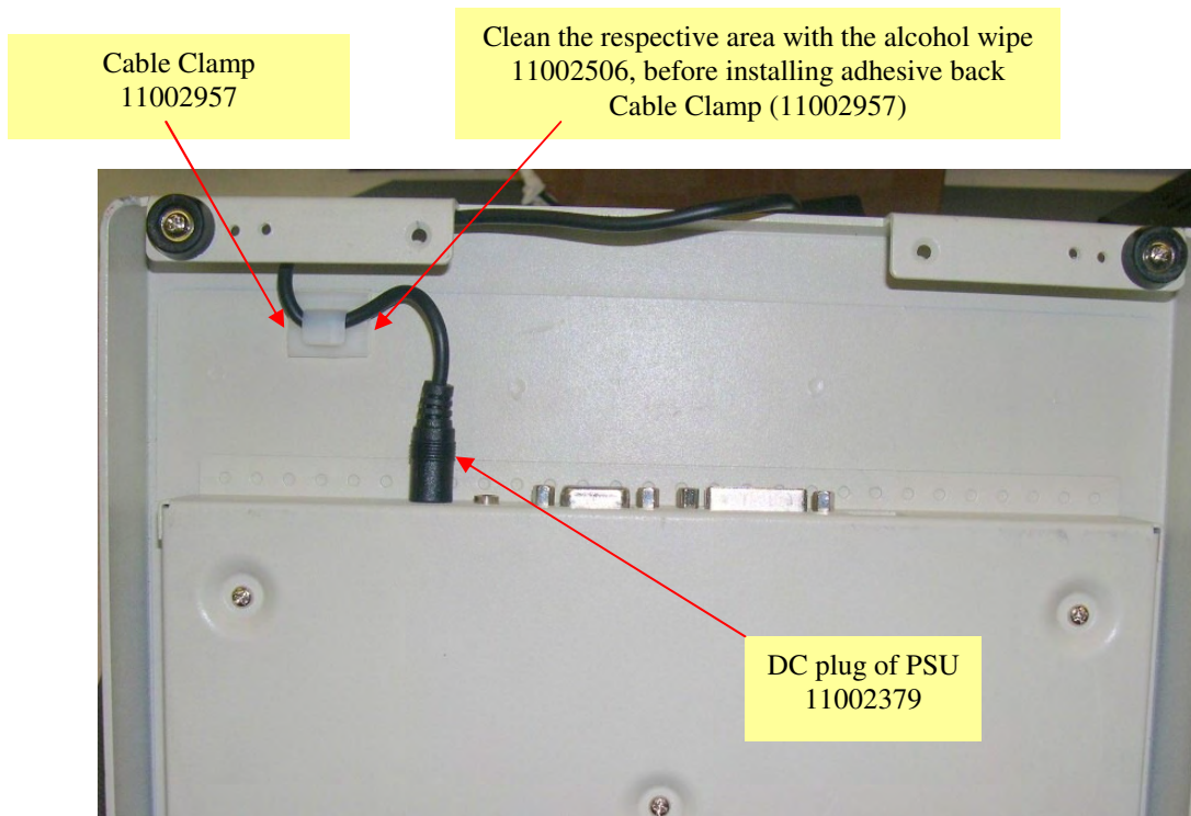
Figure 1. Installation detail
