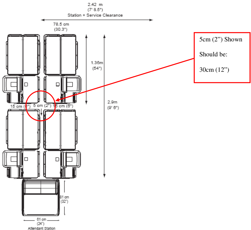
Figure 2.3 Four U-Scan4 Customer Stations with Attendant Station (C)
