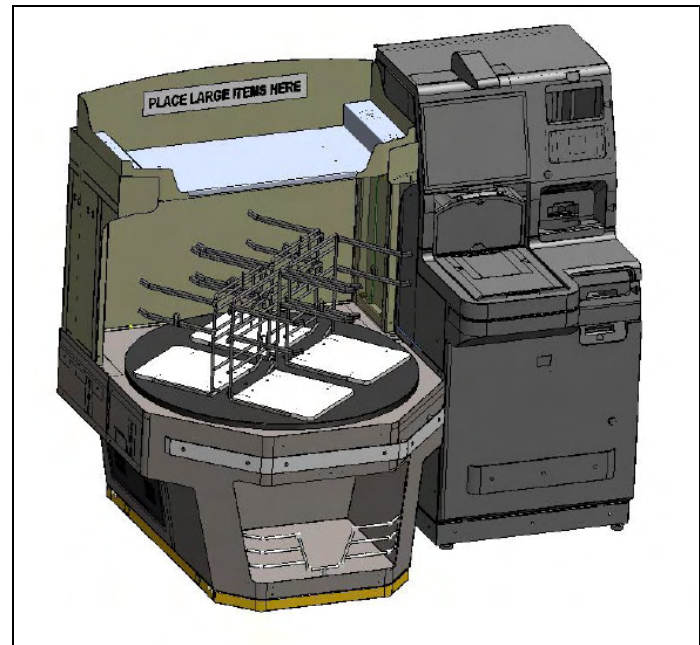
Mini-Carousel shown Attached to Genesis Robot Shown With Upper Scale
